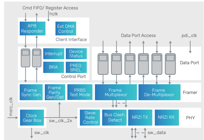
Figure 2: IP-level block diagram
