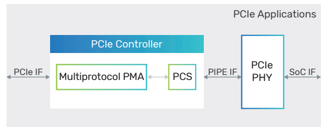
Figure 1: Example system-level block diagram
