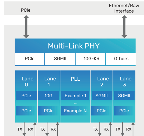
Figure 1: Example system-level block diagram
