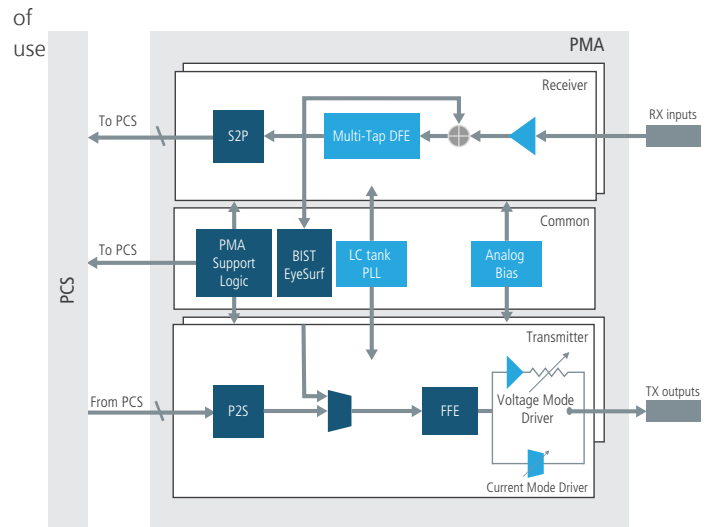
Figure 2: IP-Level Block Diagram
