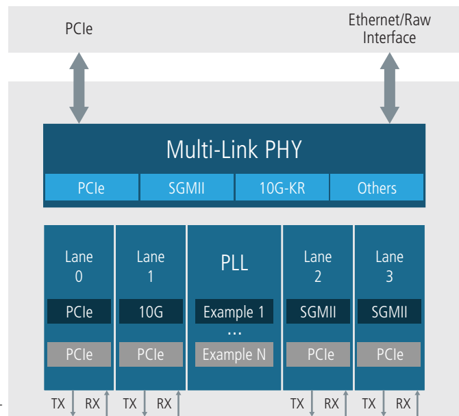
Figure 1: Example System-Level Block Diagram
