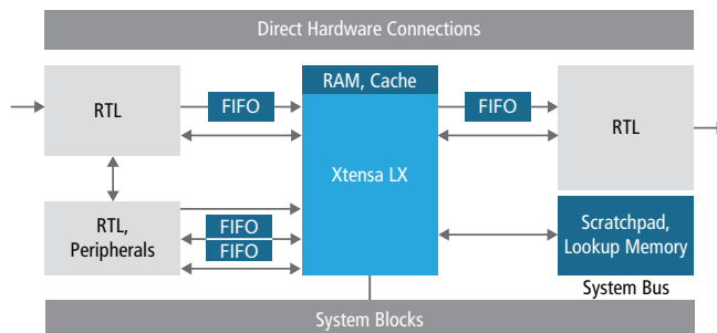
Figure 5: Example of direct FIFO and port connections using TIE queues and TIE ports
