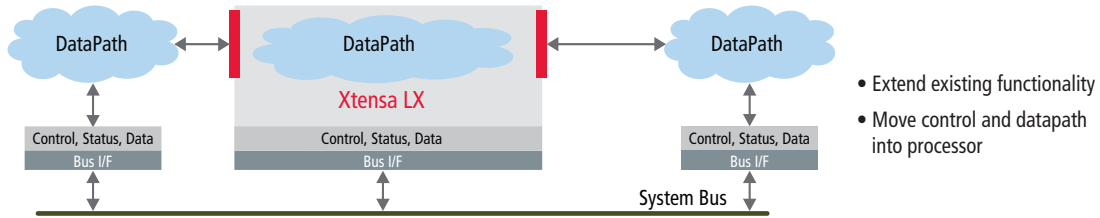
Figure 10: Both the control and datapath of the RTL block are brought into the processor
