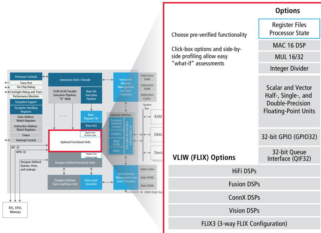
Figure 2: Widest range of configurable functional units for the Xtensa LX7 Processor
