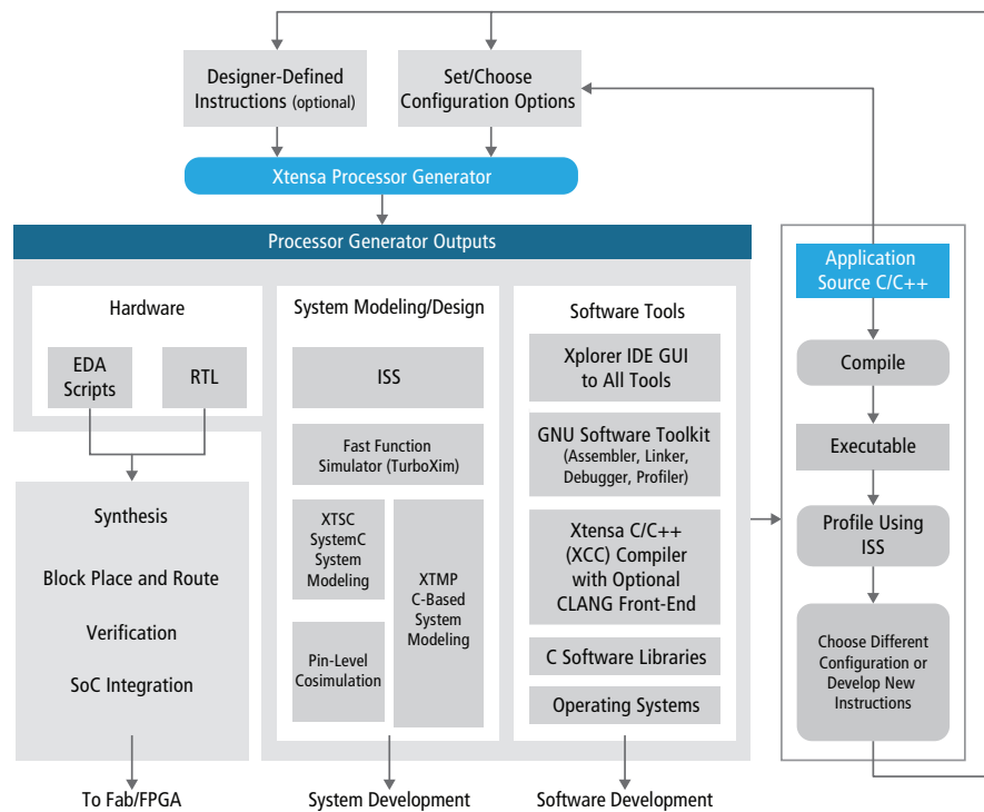
Figure 11: This proven methodology automates the creation of customized processors and matching software tools
