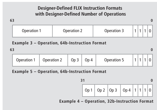
Figure 4: Designers can use FLIX to create VLIW instructions up to 128 bits wide to execute 2 to 30 parallel execution units
