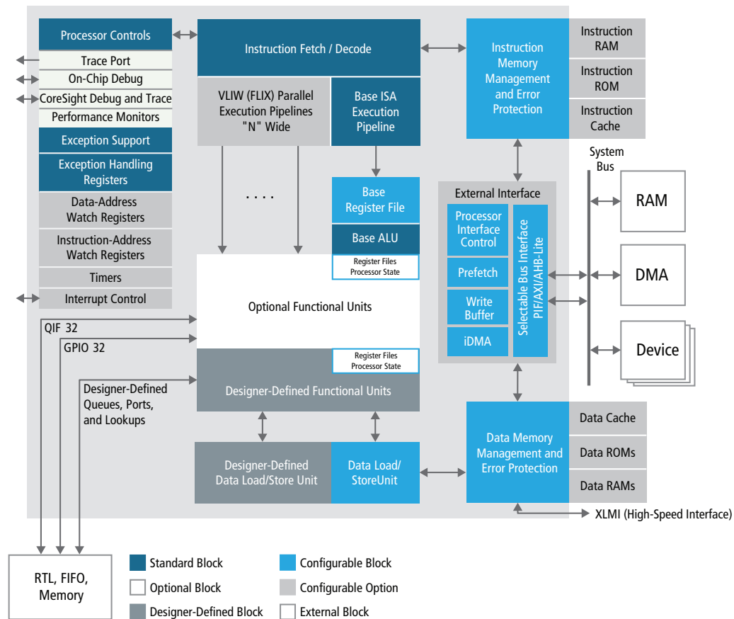
Figure 1: Block diagram of Xtensa LX7 processor architecture
