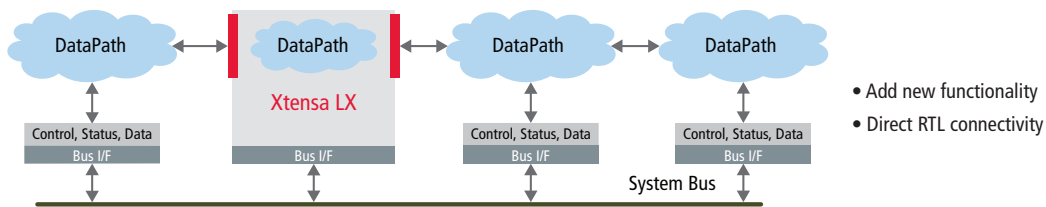
Figure 8: Direct connectivity to RTL through ports and queues
