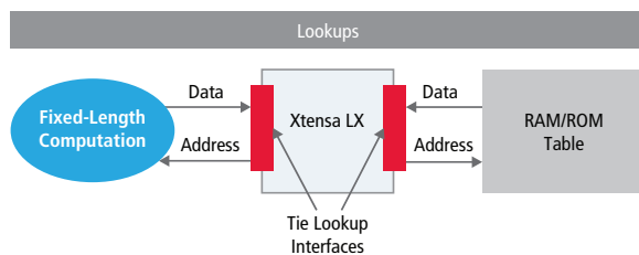
Figure 6: Example of TIE lookups showing connections to memory and logic
