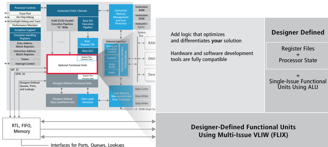
Figure 3: The Xtensa LX7 processor offers a proven method of adding designer-defined functional units and interfaces
