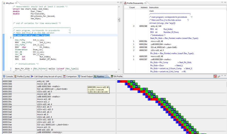
Figure 13: Xtensa Xplorer IDE GUI shows debug/trace, profiling of pipeline utilization, and a cycle comparison for a multiple core simulation
